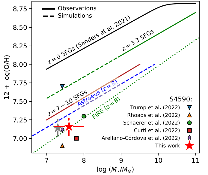
Figure 2. MZ relation of S04590. For comparison, we show the various preexisting MZ estimates for S04590 from the literature, which highlights the uncertainties from the various methods used. We also show various MZ relations either observed for galaxies at z \approx 0 and z \approx 3.3 (black and green, respectively; Sanders et al. 2021) and at z \approx 7-10 (Heintz et al. 2022b) or predicted from the Astraeus (Ucci et al. 2023) and FIRE (Ma et al. 2016) simulations, extrapolated to z \approx 8 . The local, metal-poor galaxy I Zw 18 is marked by a gray star symbol, showing an MZ relation consistent with that of S04590. Both are consistent with the predictions for high- z MZ relations.
