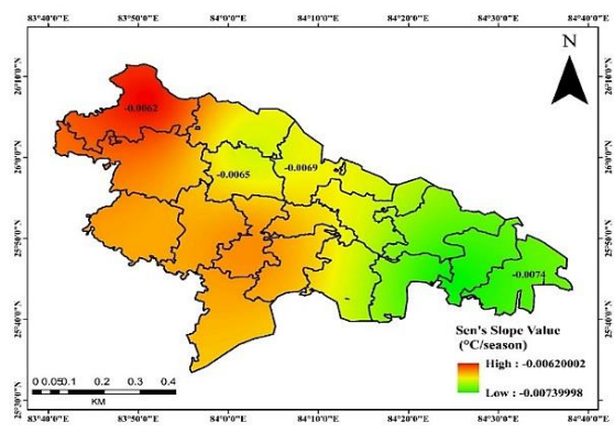
Fig. 12. Sen's slope map of maximum temperature during monsoon period in Ballia District
