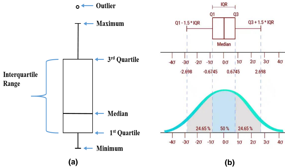
Fig. 2. (a) Five components of Box-whiskers plot (b) outliers and interquartile range
