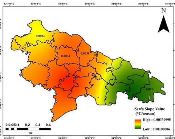
Fig. 19. Sen's slope map of minimum temperature during post-monsoon period in Ballia District
