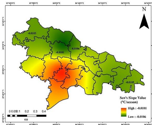
Fig. 17. Sen's slope map of minimum temperature during pre-monsoon period in Ballia District
