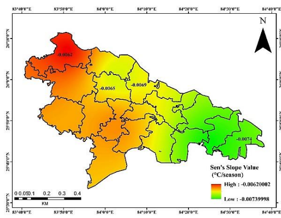
Fig. 18. Sen's slope map of minimum temperature during monsoon period in Ballia District
