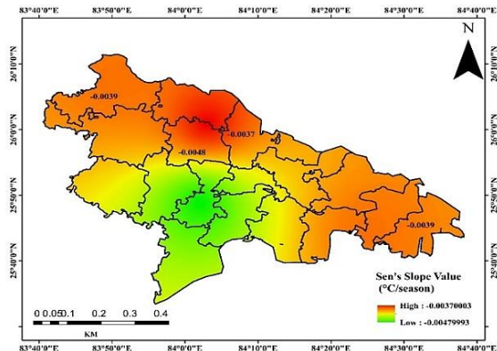
Fig. 10. Sen's slope map of maximum temperature during winter season in Ballia District
