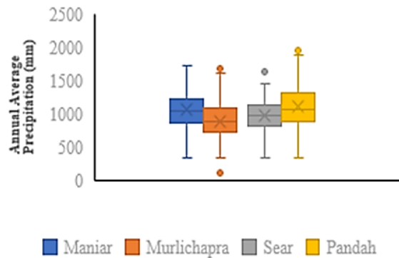
Fig. 8. Box- Plot for the precipitation (1917-2016) for all the 4-grid locations
