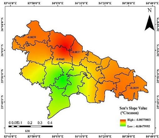
Fig. 16. Sen's slope map of minimum temperature during winter season in Ballia District
