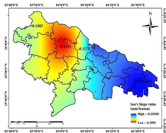
Fig. 4. Sen's slope map for the winter precipitation of Ballia District
