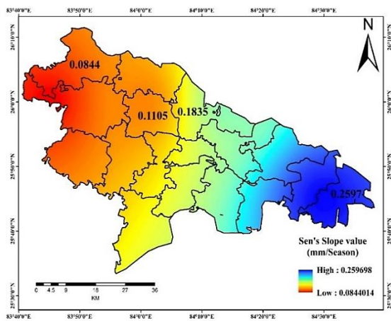
Fig. 5. Sen's slope map for the pre-monsoon precipitation of Ballia District
