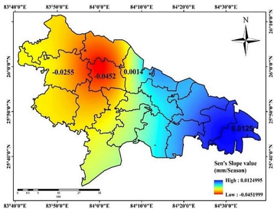
Fig. 7. Sen's slope map for the post-monsoon precipitation of Ballia District
