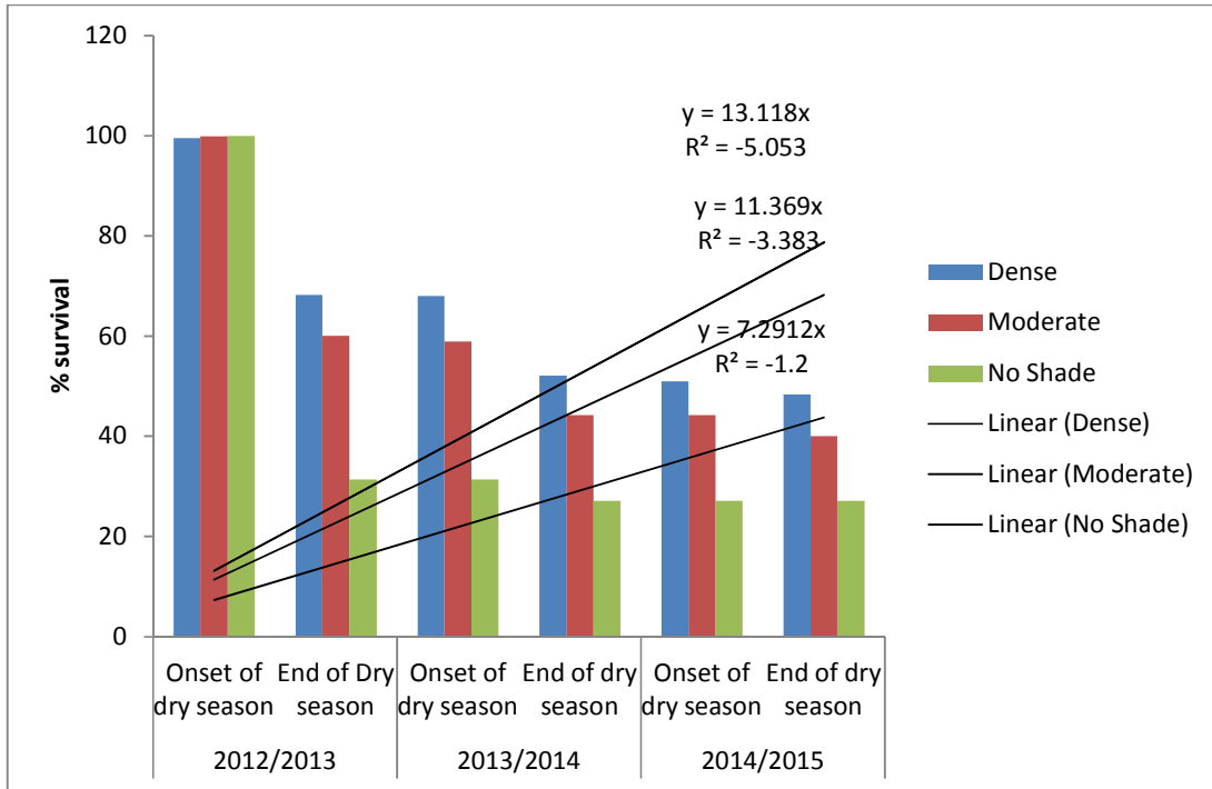
Fig. 1. Effects of shade regimes on percent survival of cacao at the onset and end of dry seasons
