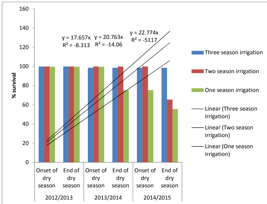
Fig. 3. Effects of varying seasons of irrigation on percent stand survival of cacao at onset and end of dry seasons
