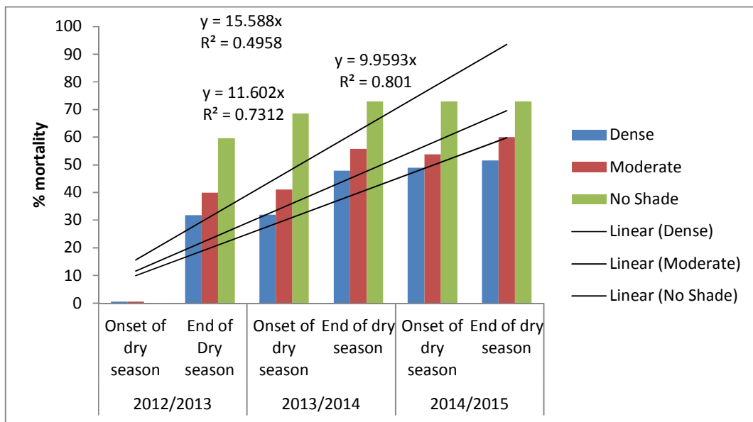
Fig. 2. Effects of shade regimes on percent stand mortality of cacao at onset and end of dry seasons
