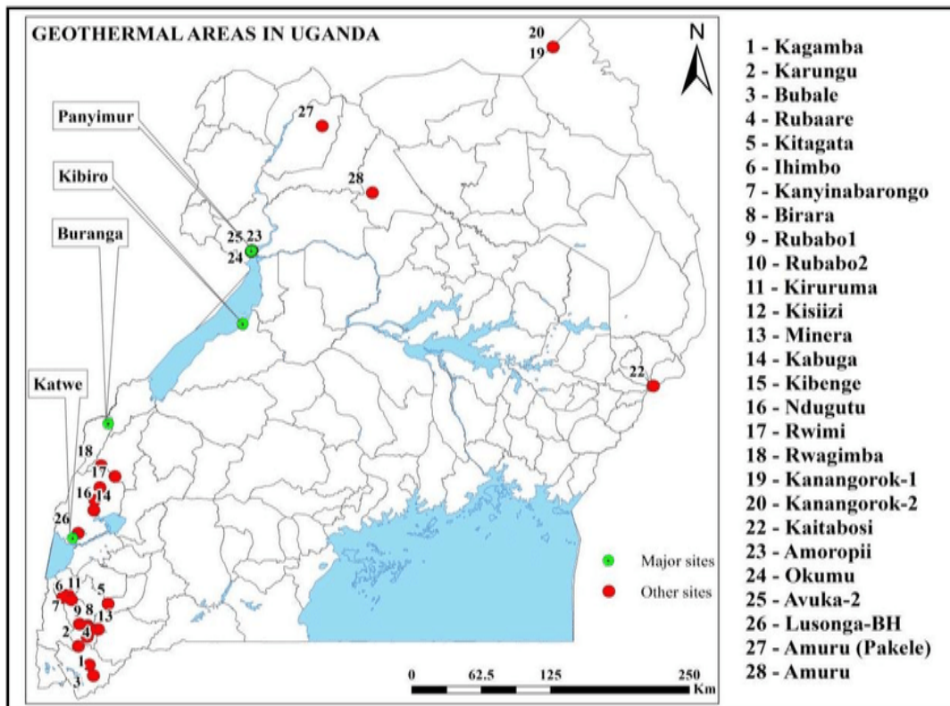
Fig. 3. Map of Uganda locating geothermal energy resources
