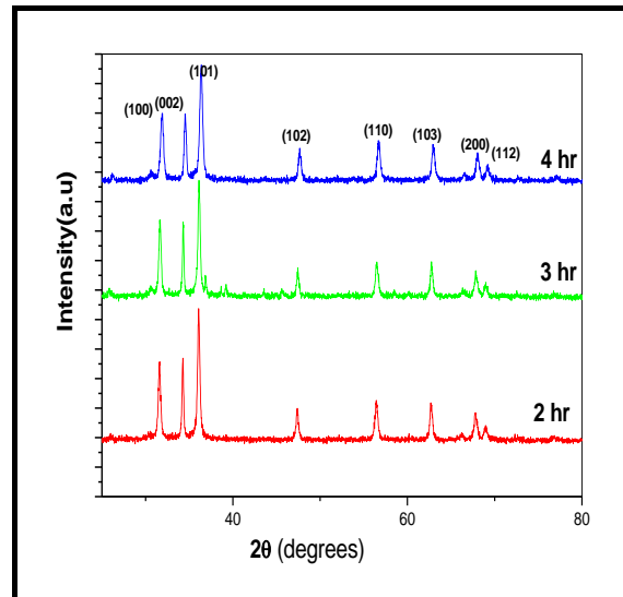
Figure (2): XRD patterns of ZnO nanoparticles sonicated at 2, 3 and 4 hours.
