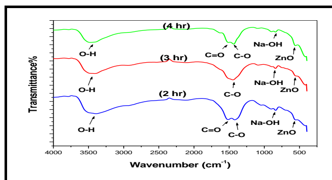
Figure (5): FTIR spectra of samples sonicated for 2, 3 and 4 hours.
