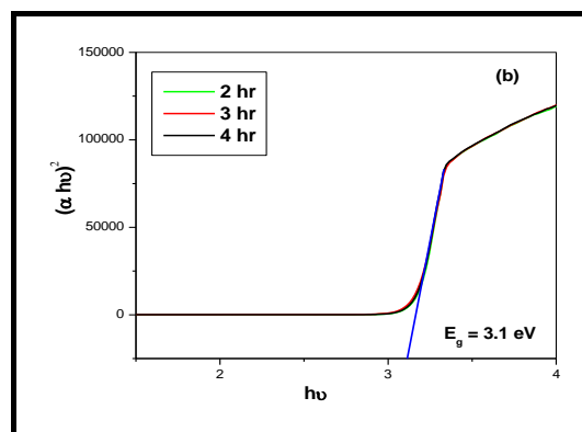
Figure 6: (a) Absorption spectra and (b) The relation between (\alpha h\nu)^2 versus h\nu for 2, 3 and 4 samples.
