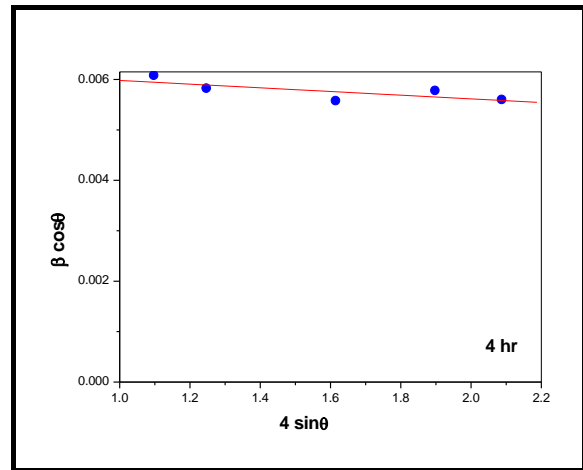
Figure (3): The W-H analysis using UDM of ZnO nanoparticles sonicated at 2, 3 and 4 hours.
