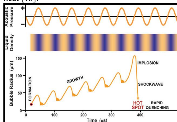
Figure (1): Formation, growth and implosion of bubbles during the sonochemical method.
