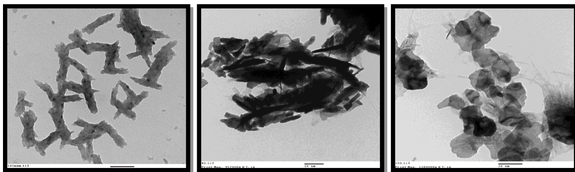
Figure (4): TEM images for samples sonicated for 2, 3 and 4 hours.
