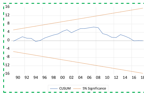
(a) Cumulative sum (CUSUM) test output
