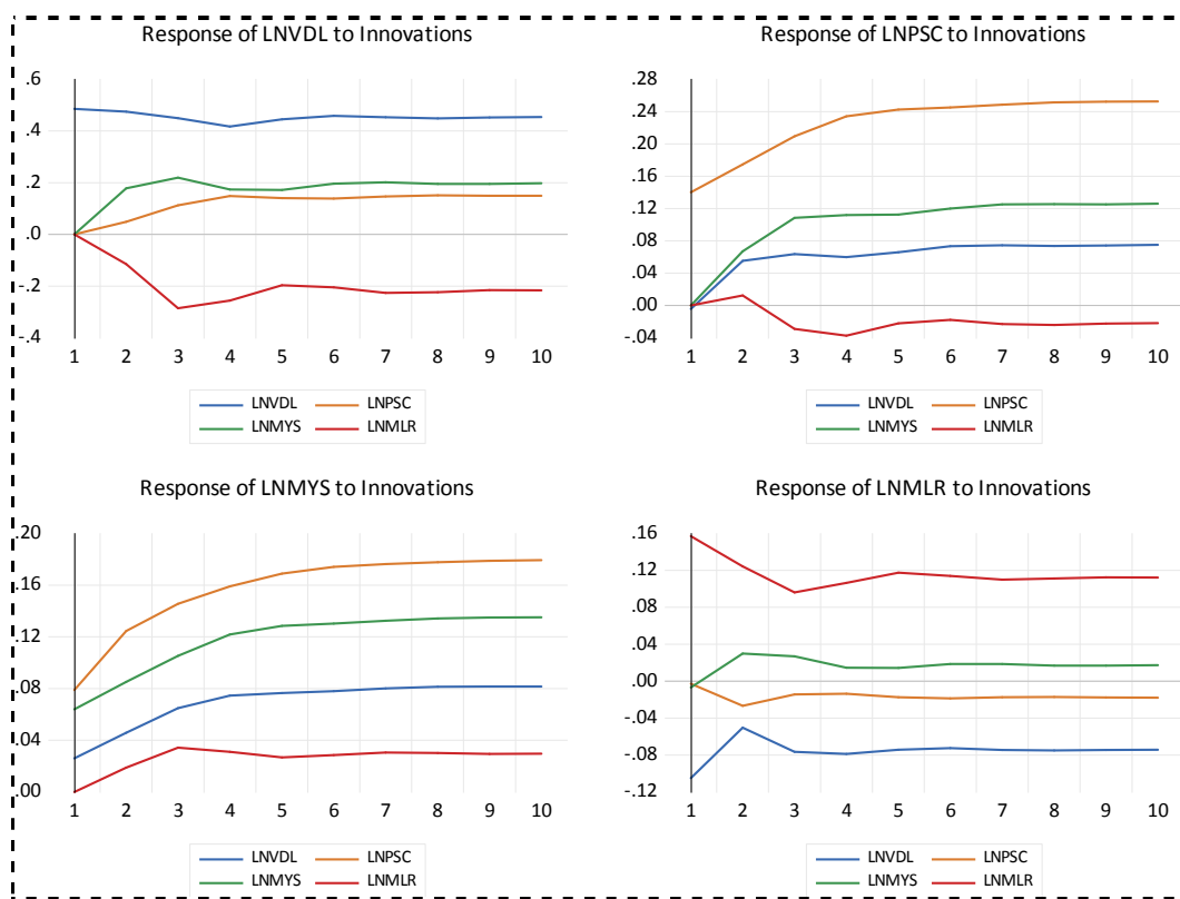
Fig. 4. Response of included variables to Cholesky one standard deviation innovations
