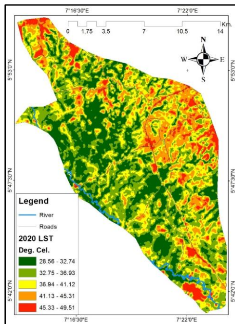
Fig. 11. Spatial distribution of land surface temperature in 2020
