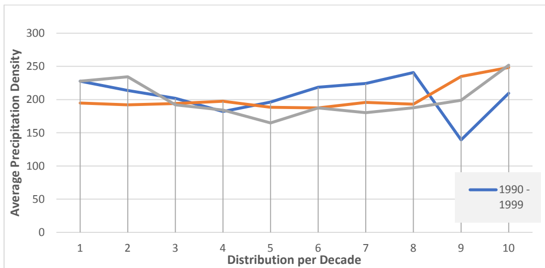
Fig. 15. Three decadal trends of precipitation density in the study area
