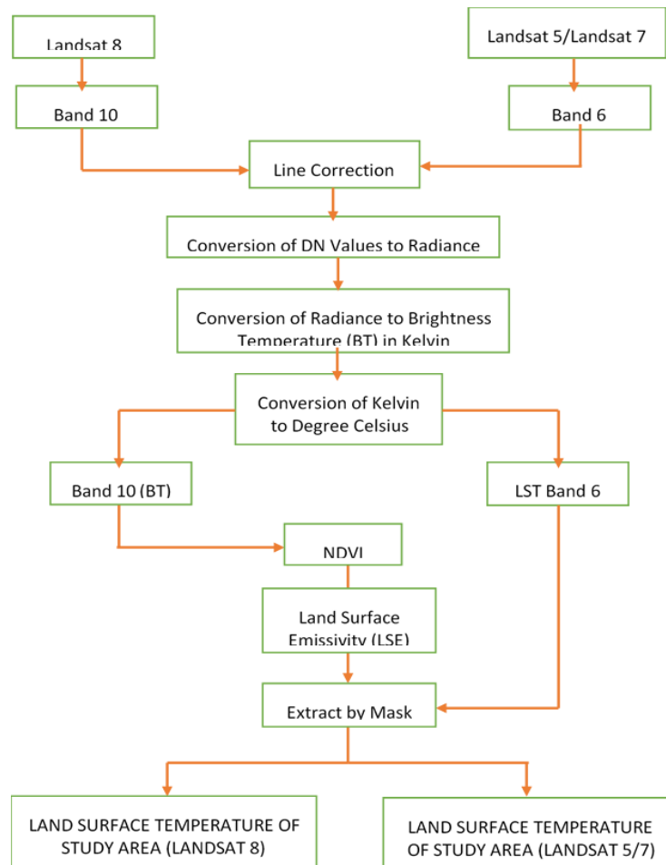
Fig. 3. Land Surface Temperature Analysis Flow [28]
