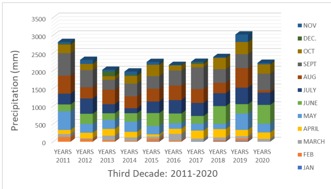
Fig. 14. Temporal trends in precipitation for the study area 2011 – 2020
