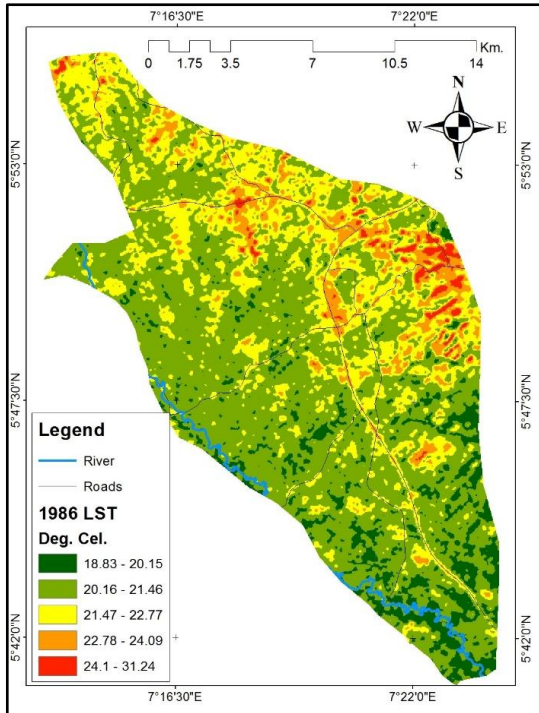
Fig. 9. Spatial Distribution of Land Surface Temperature in 1986
