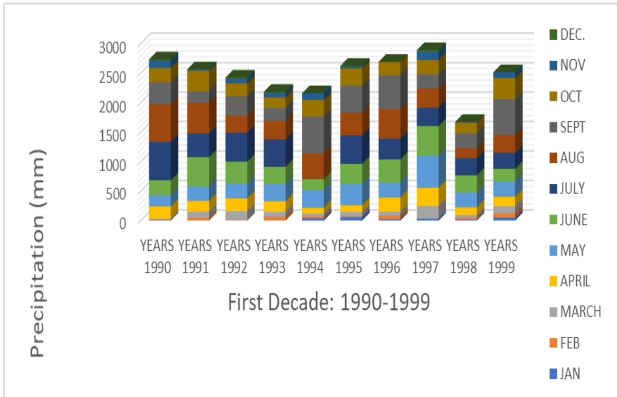
Fig. 12. Temporal trends of precipitation for the study area 1990 – 1999
