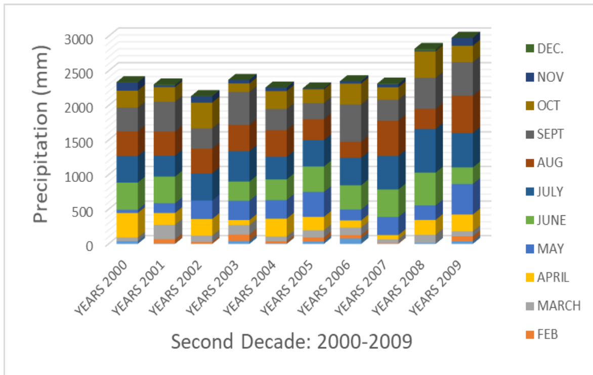
Fig. 13. Temporal trends of precipitation for the study area 2000 – 2009
