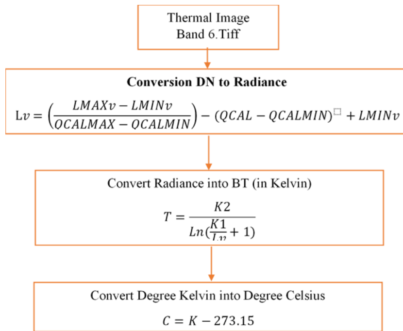
Fig. 2. Formulas for estimating land surface temperature (LST)
