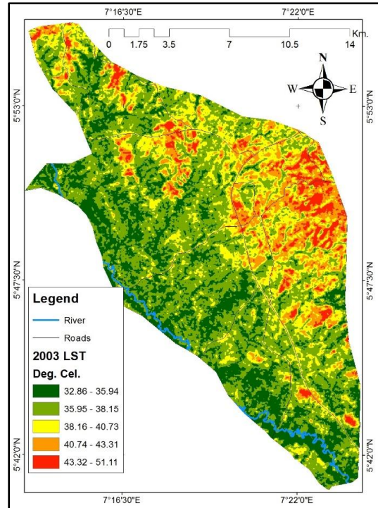
Fig. 10. Spatial Distribution of Land Surface Temperature in 2003
