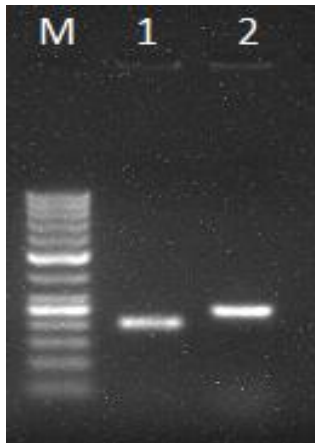
Fig. 1. PCR identification of E. coli ; Lane M: 50 bp DNA ladder, Lane 1: M12 gene fragment (200 bp), Lane 2: lacZ 4 gene fragment (243 bp)
