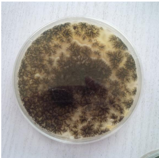
Aspergillus sp
