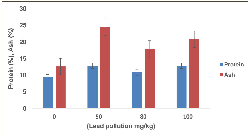
Fig. 2. Percentage protein and ash in mushrooms harvested from lead polluted soil
