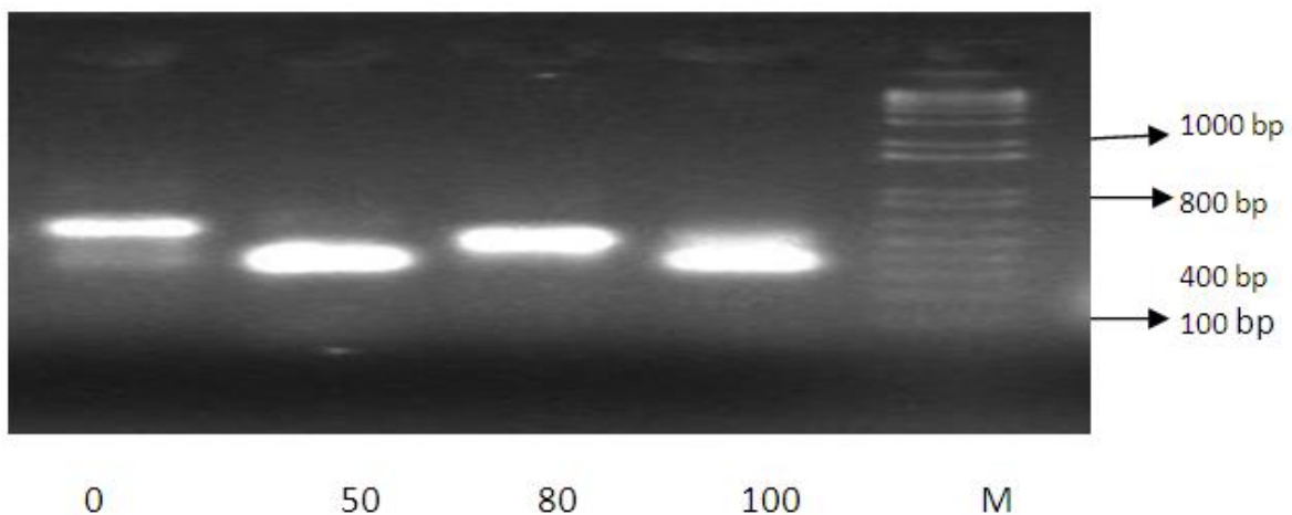
Plate 1. DNA profile of Pleurotus tuber-regium grown in lead-polluted soil (0, 50, 80, 100 mg/kg) using ITS 1/ITS 4 universal primers. Line M- 100 base pair marker
