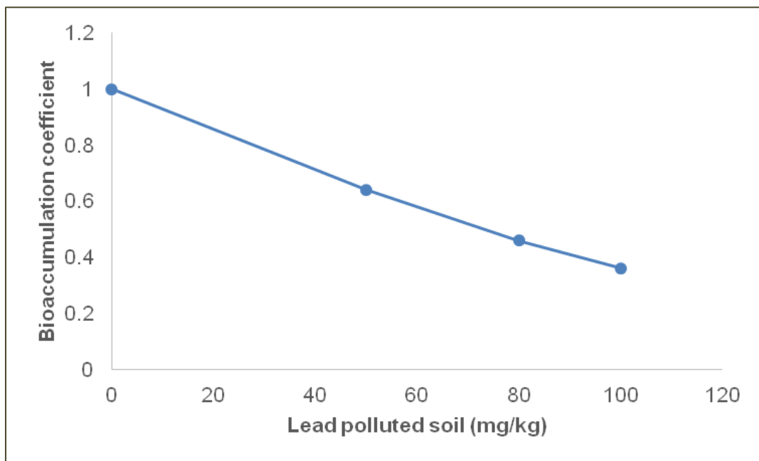
Fig. 1. Bioaccumulation coefficient of P. tuber-regium in lead continuously polluted soil
