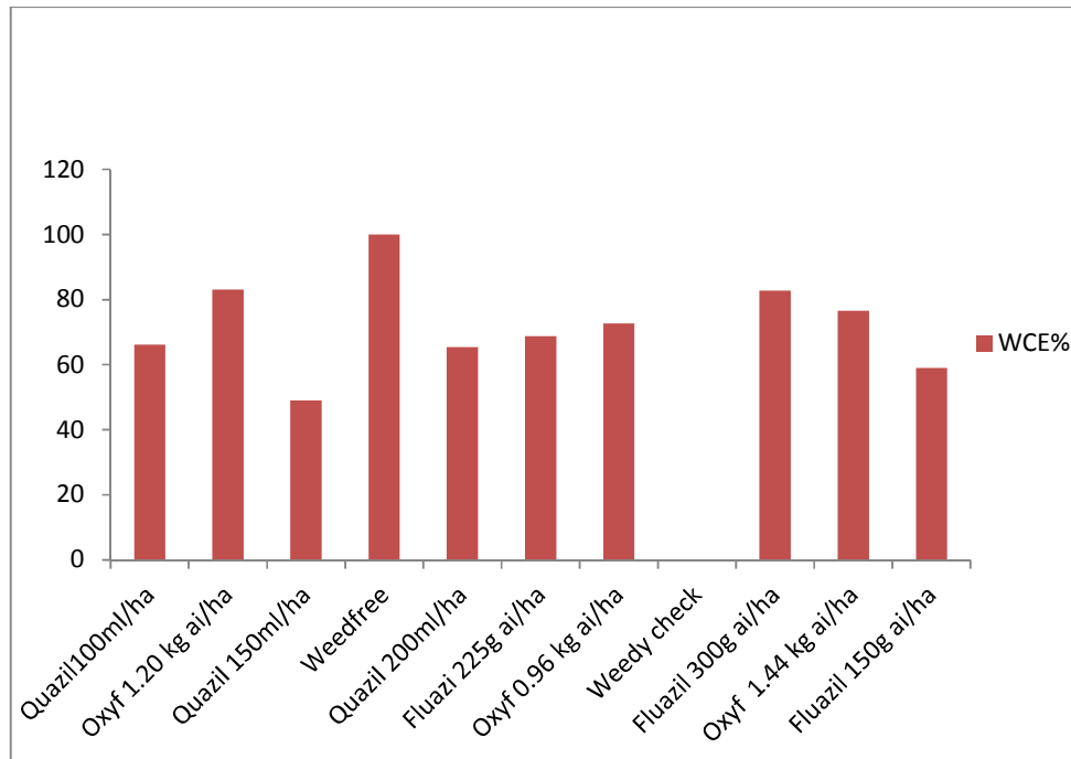
Figure 3. Weed control efficiency of herbicides
