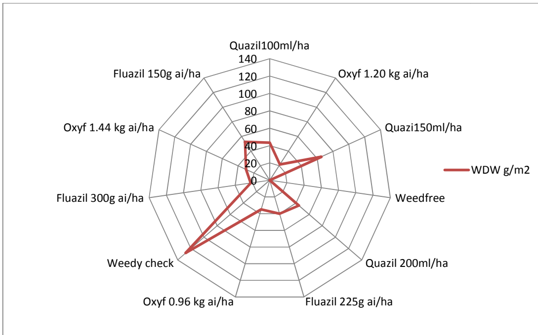
Figure 1. Effects of herbicides on weed growth at kenaf fibre harvest
