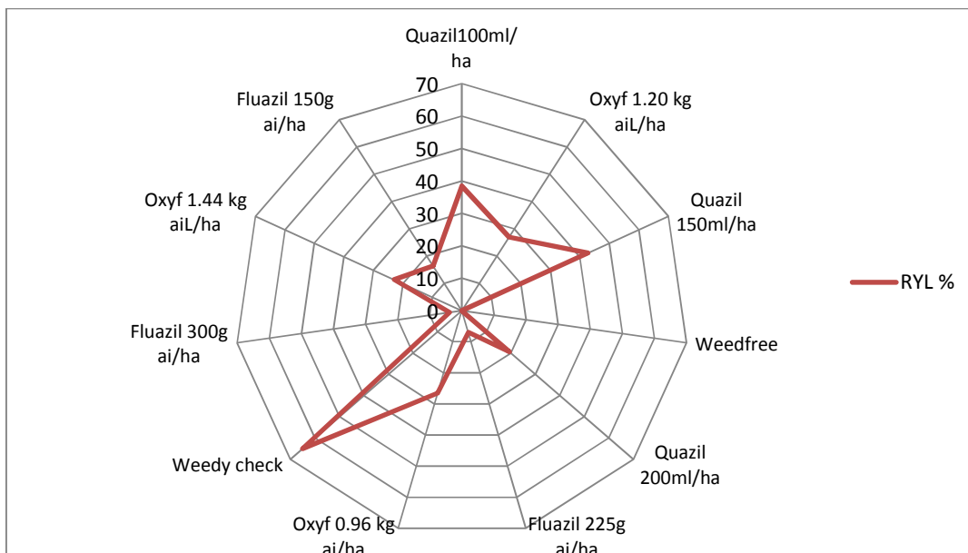
Figure 4. Effects of herbicides on kenaf relative yield loss
